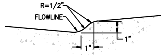
DETAIL "B"
