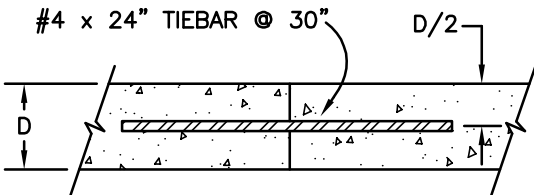
EMERGENCY CONSTRUCTION JOINT
