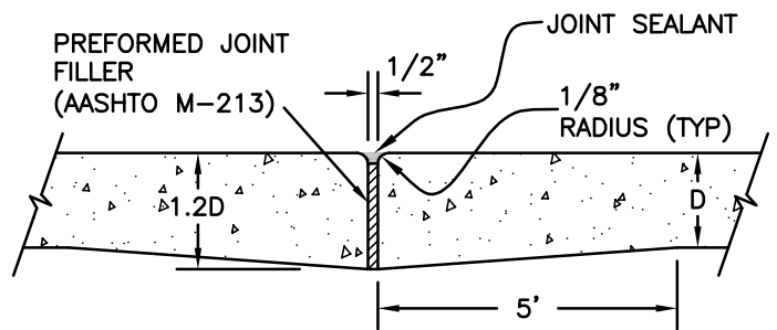
THICKENED EDGE ISOLATION JOINT
