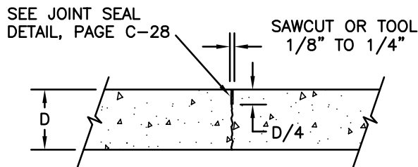
CONTRACTION JOINT
