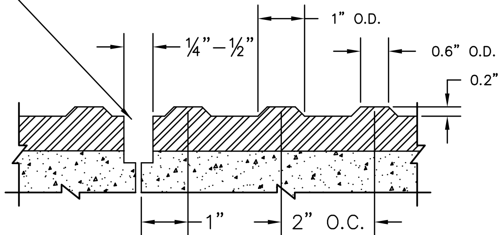
DOMES AND JOINT DETAIL
